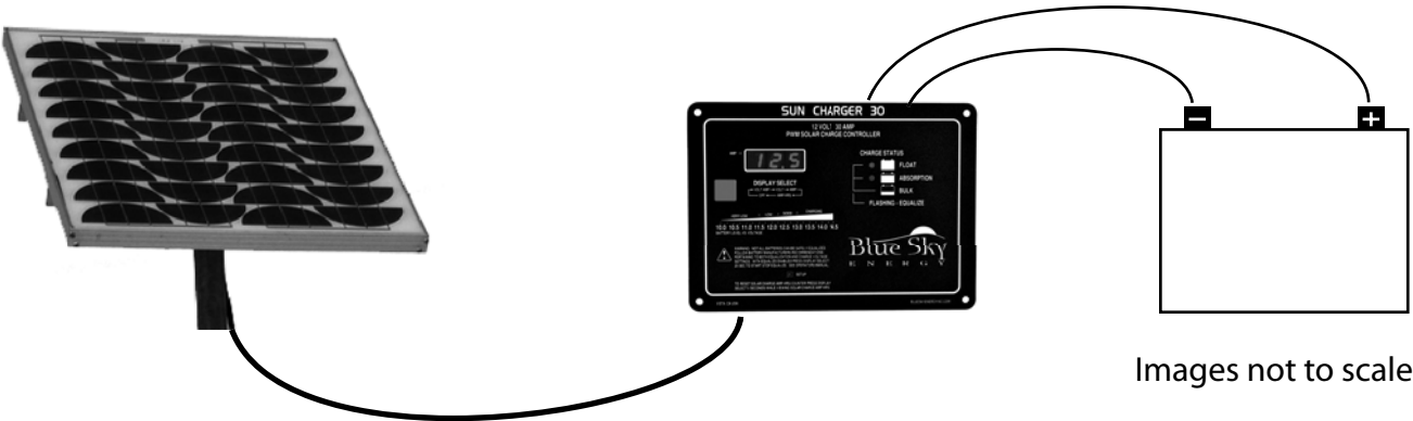
Typical illustration of solar panel to Sun Charger 30 to Battery
