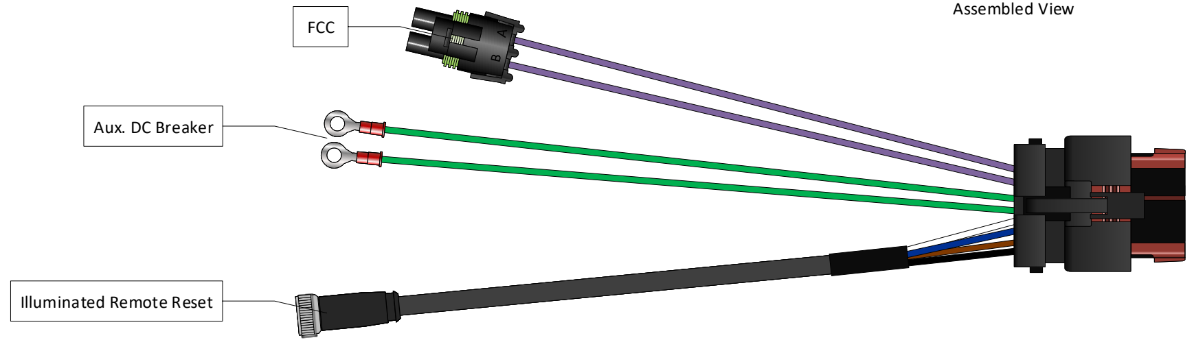
Assembled View
